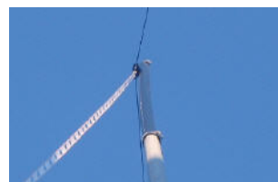
"Plastic on Metal" - Using a PVC extension to a metal mast. Note that the vertical section is kept clear of the mast.
